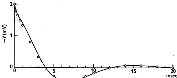
Fig. 24. Comparison of step-by-step solution and linear approximation. Eqn. (26), temperature 6^\circ\text{C} ; initial displacement of -V=2 mV. Continuous line: step-by-step solution. Circles: linear approximation with same initial displacement.
