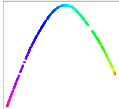
Laplacian Eigenmaps
