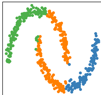
k-means: noisy.moons
