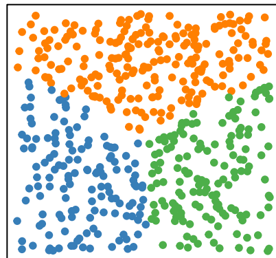
k-means: no.struct
