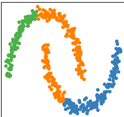
Ward: noisy.moons
