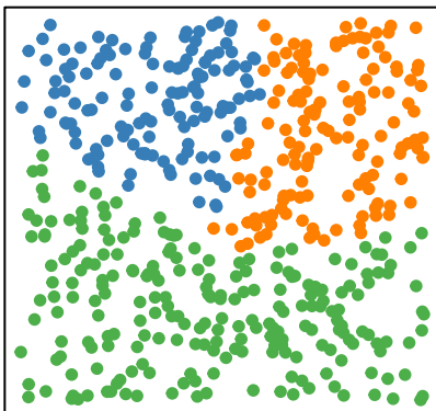
Ward: no.struct
