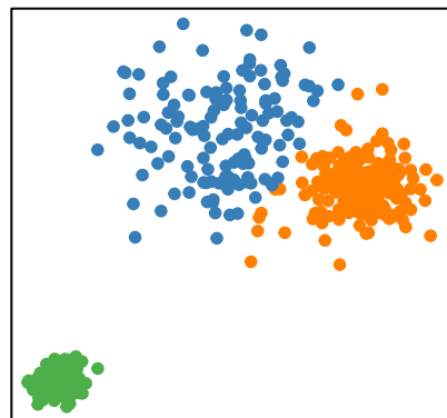
k-means: varied
