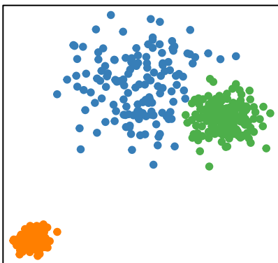
Ward: varied
